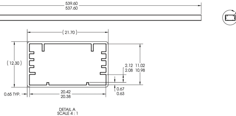
Figure 38: Tube Design for Hexagonal Star Products
